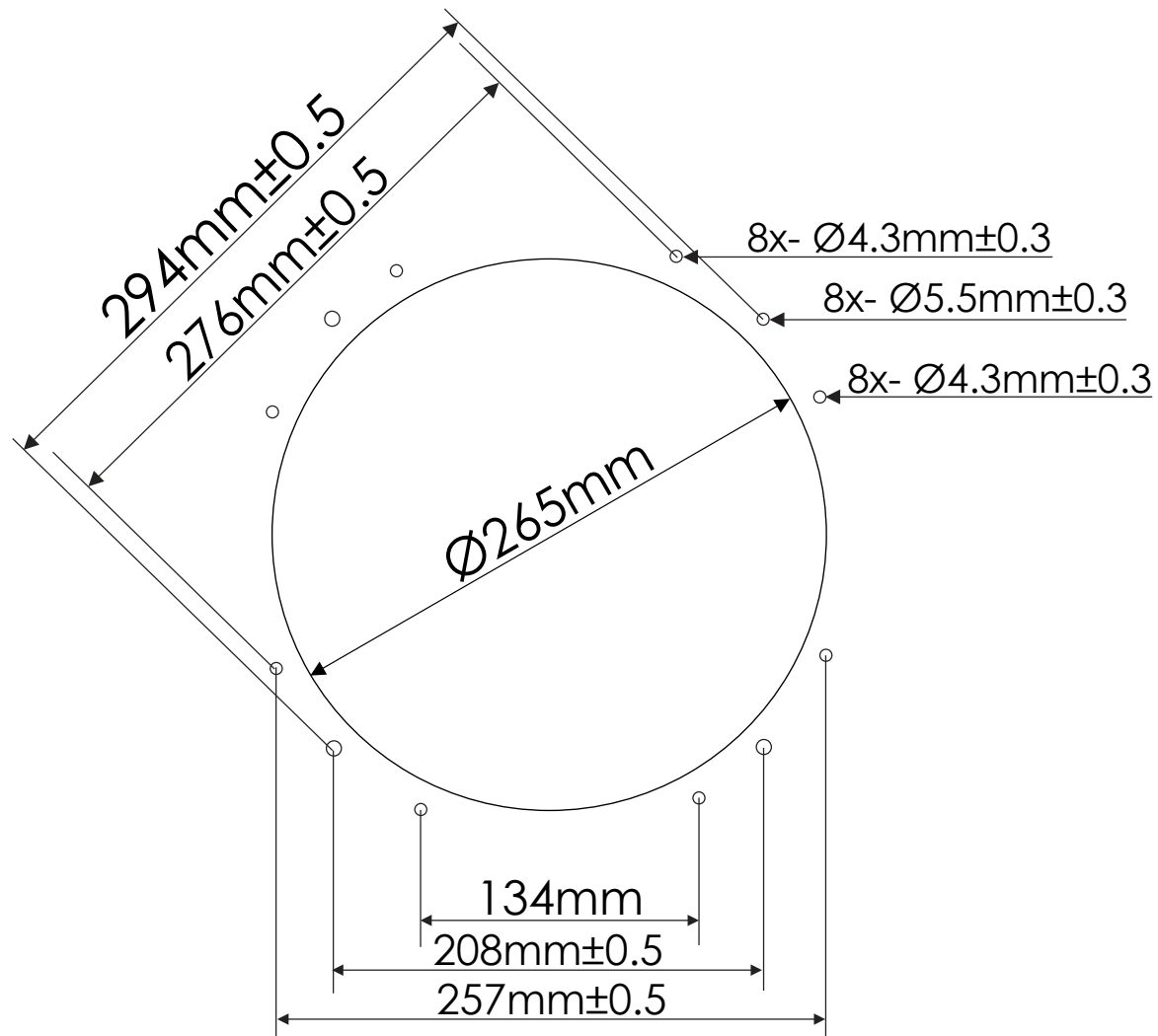
OD280 Panel Cutout Diagram
