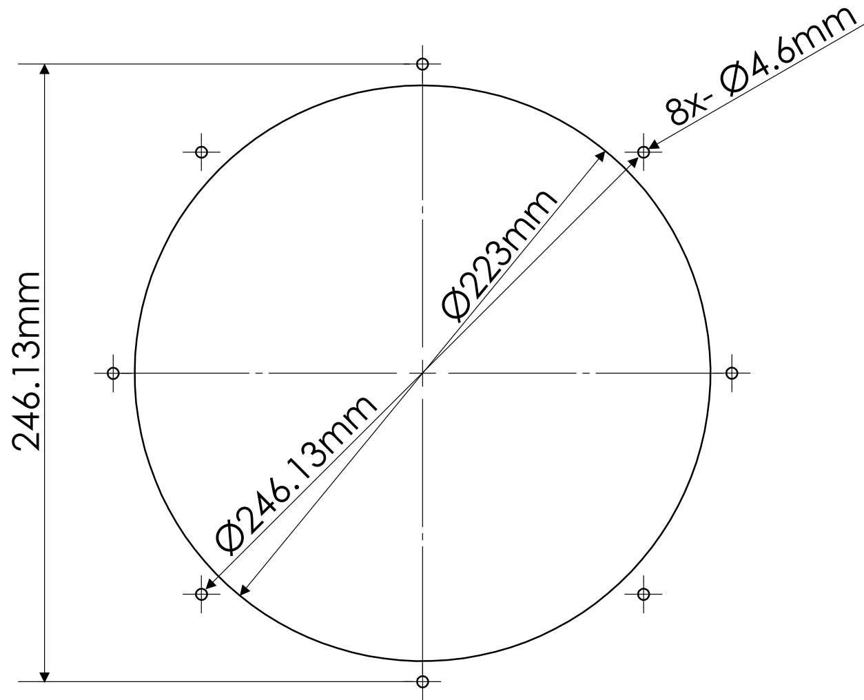
OD254AP Panel Cutout Diagram
