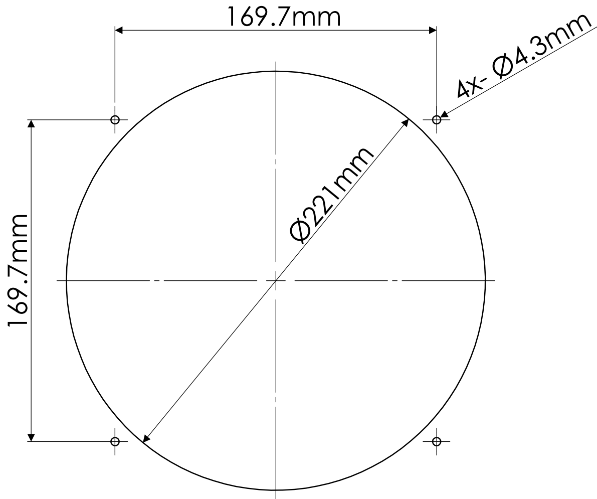
OA225AN METAL Panel Cutout Diagram
